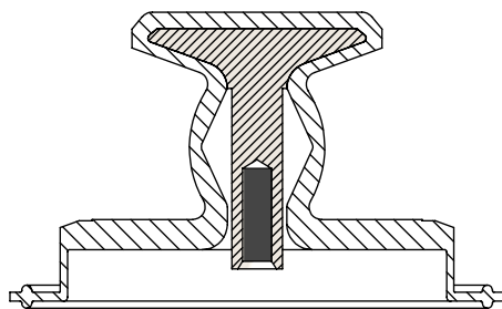
SECTION VIEW
